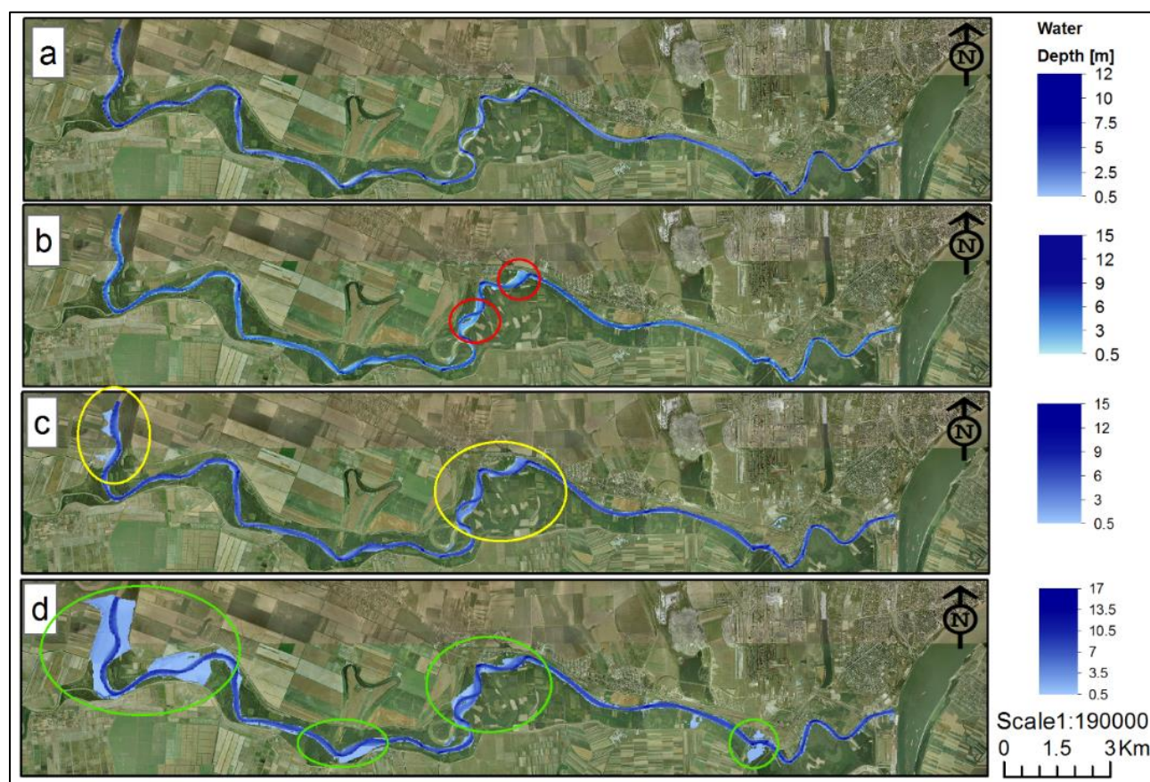
Figure 3.45. Flood scenarios and water depth: a – flow Q=500\text{ m}^3/\text{s} , b – flow Q=1000\text{ m}^3/\text{s} , c – flow Q=1500\text{ m}^3/\text{s} , d – flow N10\% Q=2280\text{ m}^3/\text{s}
